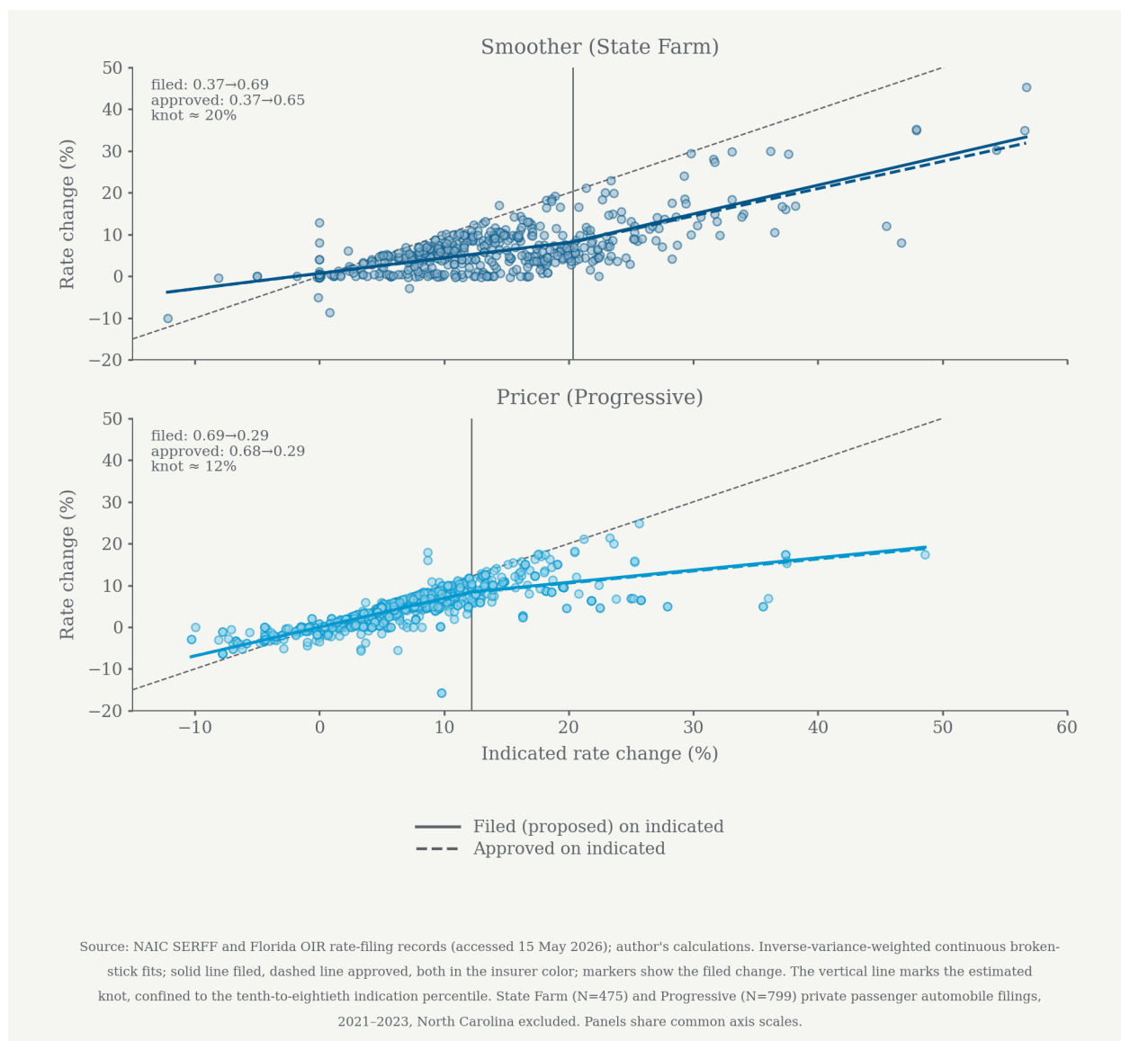
Figure C.2. Leverage-controlled pass-through on the insurers' own filed (proposed) changes, with the approved fit overlaid, on the sample excluding North Carolina; inverse-variance-weighted continuous broken-stick fits, 2021–2023, one panel per insurer. The horizontal axis is the indicated rate change in percent and the vertical axis the rate change in percent; the dashed gray line is the 45-degree identity and the vertical line marks the estimated knot. Both fits are drawn in the insurer's color: the solid line is the fit to the filed change and the dashed line the fit to the approved change; markers show the filed change. The estimator and the tenth-through-eightieth-percentile knot restriction match Figure 4. State Farm N = 475 , Progressive N = 799 ; North Carolina excluded. Source: SERFF and Florida OIR (accessed 15 May 2026); author's calculations.
