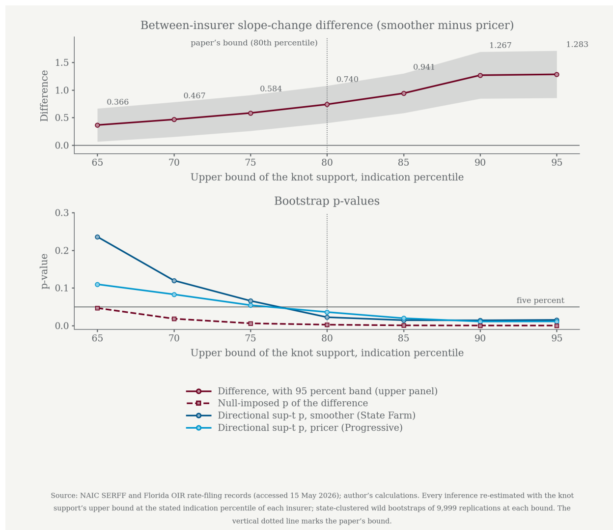
Figure B.3. The between-insurer inference across the upper bound of the knot support, filed change, 2021–2023. The horizontal axis of both panels is the upper bound of the knot support as an indication percentile of each insurer's sample, from the sixty-fifth through the ninety-fifth; the dotted vertical line marks the paper's eightieth. The upper panel plots the difference in slope changes, smoother minus pricer, at the knot each bound selects, with its 95 percent band from the cluster-robust standard error, and labels each value. The lower panel plots three bootstrap p -values against the five percent line: the null-imposed p -value of the difference (maroon, dashed), and the directional supremum- t p -values of the smoother (State Farm, deep blue) and the pricer (Progressive, bright blue), each from a state-clustered wild bootstrap of 9,999 replications at that bound. State Farm N = 477 , Progressive N = 802 . Source: SERFF and Florida OIR (accessed 15 May 2026); author's calculations. The difference rises with the bound and rejects at every bound; the directional tests cross five percent between the seventy-fifth and the eightieth percentile.
