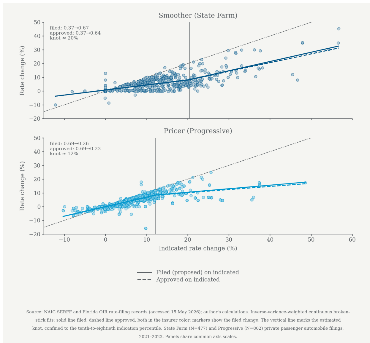
Figure 4. Leverage-controlled pass-through on the insurers' own filed (proposed) changes, with the approved fit overlaid; inverse-variance-weighted continuous broken-stick fits, 2021–2023, one panel per insurer. The horizontal axis is the actuarially indicated rate change in percent and the vertical axis the rate change in percent; the dashed gray line is the 45-degree identity and the vertical line marks the estimated knot. Both fits are drawn in the insurer's color, matching Figure 3: the solid line is the fit to the filed change and the dashed line the fit to the approved change. Markers show the filed change. The fit is feasible generalized least squares with weights set to the inverse of a locally estimated variance from a robust LOWESS mean, so the sparse, high-variance high-indication filings are downweighted in estimation (Appendix B); the knot is confined to the tenth-through-eightieth indication percentile. The filed change is floored at the approved change for the small share of filings that record a proposed below the approved. State Farm N = 477 , Progressive N = 802 . Source: SERFF and Florida OIR (accessed 15 May 2026); author's calculations.
