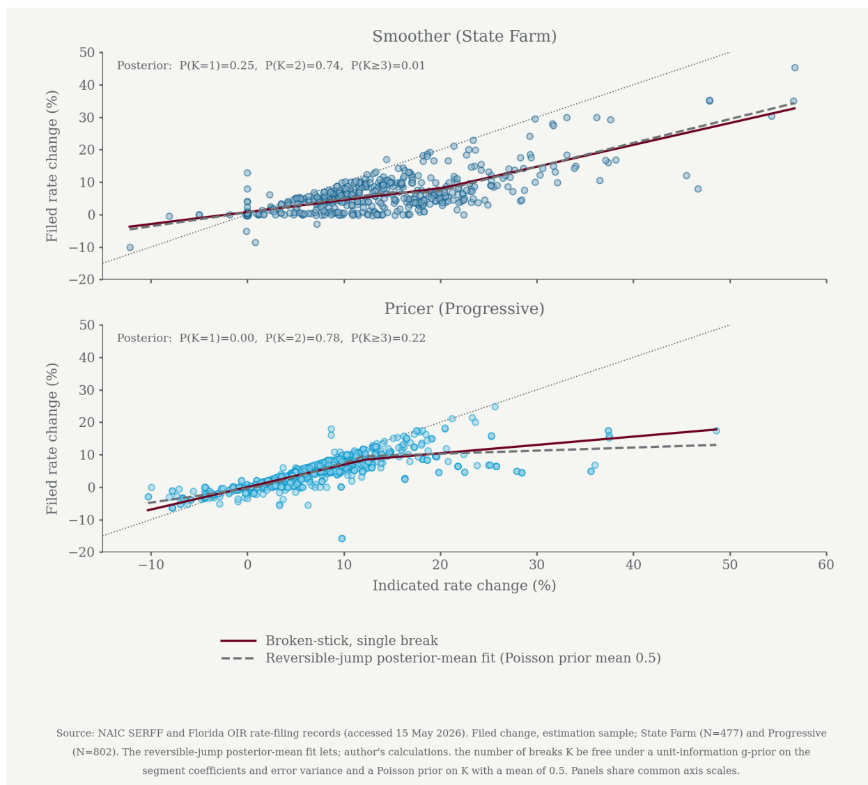
Figure B.2. Sensitivity of the pass-through curvature to freeing the number of breaks, filed change, 2021–2023, one panel per insurer, the smoother (State Farm) above the pricer (Progressive). The horizontal axis is the indicated rate change in percent and the vertical axis the filed rate change in percent, on scales common to both panels; the dotted line is the 45-degree identity. Points are filings in the insurer's color. The solid line is the inverse-variance-weighted broken-stick fit with a single break, the primary specification of Figure 4; the dashed line is the posterior-mean fit of a reversible-jump sampler that lets the number of breaks K be free, under a unit-information g -prior on the segment coefficients and error variance and a Poisson prior on K with a mean of one-half. Knot locations are supported on the tenth-through-eightieth indication percentile, at most four breaks are entertained, and each segment is required to hold at least fifteen filings; the chain is run for 80,000 draws from a fixed seed, of which the first 20,000 are discarded. The annotation in each panel reports the posterior probability of K breaks. State Farm N = 477 , Progressive N = 802 . Source: SERFF and Florida OIR (accessed 15 May 2026); author's calculations. The posterior-mean fit tracks the broken-stick and preserves the convex pass-through of the smoother and the concave pass-through of the pricer.
