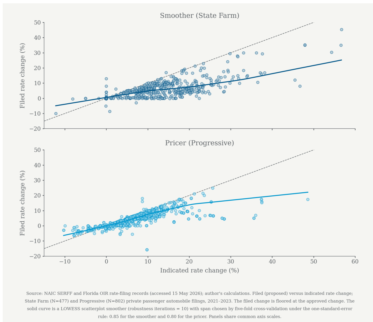
Figure 3. Filed versus indicated rate change at the filing level, 2021–2023, one panel per insurer. The horizontal axis is the indicated rate change in percent; the vertical axis is the filed (proposed) rate change in percent; the dashed line is the 45-degree identity. The solid curve is a LOWESS scatterplot smoother (Cleveland 1979) with robustness iterations set to ten and span selected by five-fold cross-validation under the one-standard-error rule (Hastie, Tibshirani, and Friedman 2009), span 0.85 for the smoother and 0.80 for the pricer. State Farm N = 477 , Progressive N = 802 . Source: SERFF and Florida OIR (accessed 15 May 2026); author's calculations. The scatterplot smoother bends downward at high indication for the pricer and is closer to linear for the smoother.
