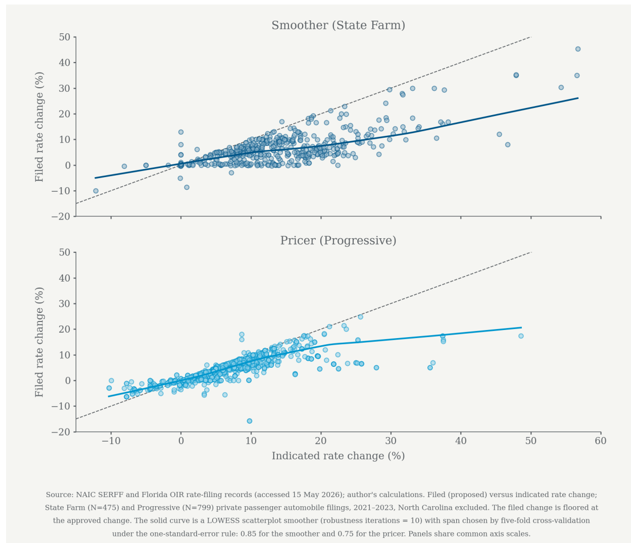
Figure C.1. Filed versus indicated rate change at the filing level on the sample excluding North Carolina, 2021–2023, one panel per insurer. The horizontal axis is the indicated rate change in percent; the vertical axis is the filed (proposed) rate change in percent; the dashed line is the 45-degree identity. The solid curve is a LOWESS scatterplot smoother (Cleveland 1979) with robustness iterations set to ten and span selected by five-fold cross-validation under the one-standard-error rule (Hastie, Tibshirani, and Friedman 2009), span 0.85 for the smoother and 0.75 for the pricer. State Farm N = 475 , Progressive N = 799 ; North Carolina excluded. Source: SERFF and Florida OIR (accessed 15 May 2026); author's calculations. The scatterplot smoother bends downward at high indication for the pricer and is closer to linear for the smoother, as in Figure 3.
