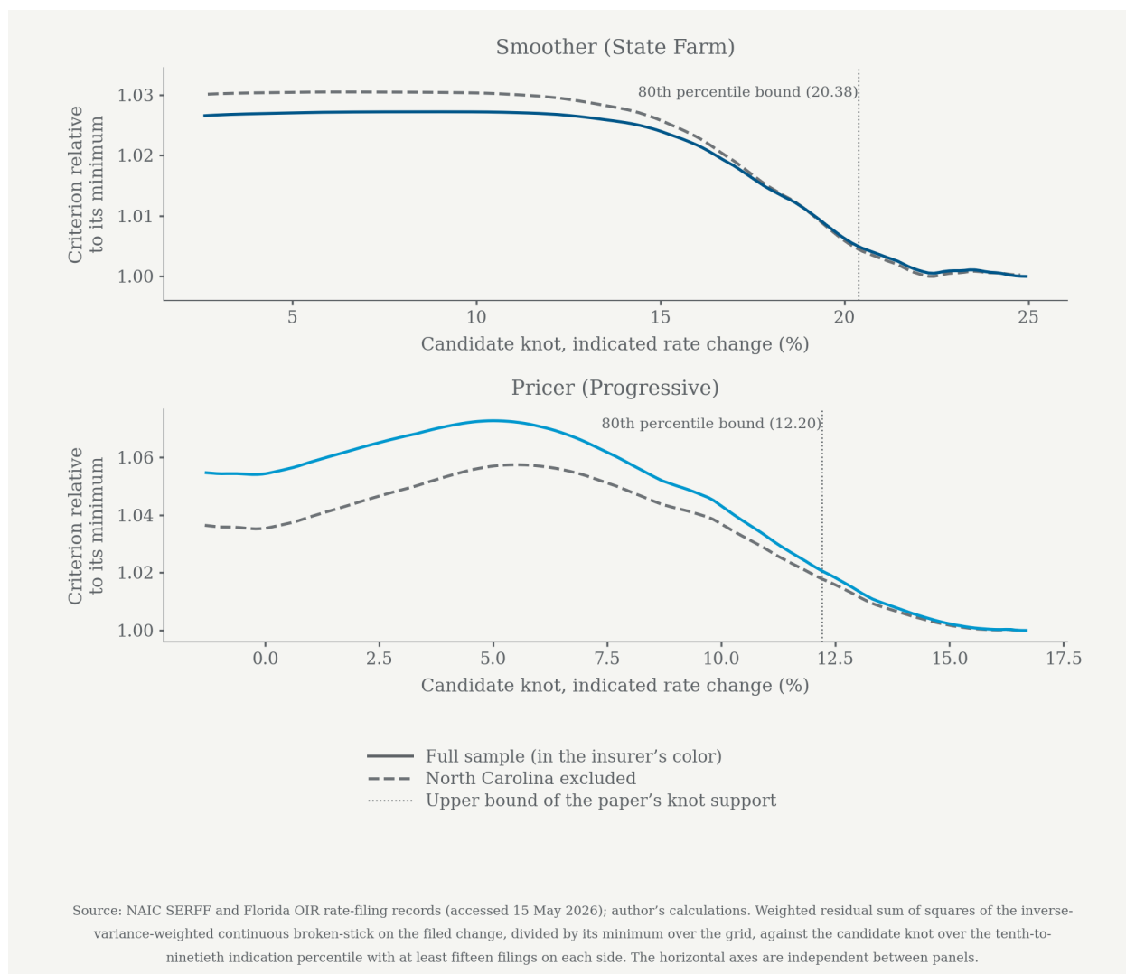
Figure B.1. Criterion profile of the broken-stick knot search, filed change, 2021–2023, one panel per insurer, the smoother (State Farm) above the pricer (Progressive). The horizontal axis is the candidate knot in percent of indicated rate change, on an independent scale per panel; the vertical axis is the weighted residual sum of squares of the inverse-variance-weighted continuous broken-stick at that knot, divided by its minimum over the grid. The solid line in the insurer's color is the full sample and the dashed gray line the sample excluding North Carolina; the dotted vertical line marks the upper bound of the paper's knot support, the eightieth indication percentile of the full sample, and the grid runs from the tenth through the ninetieth percentile with at least fifteen filings on each side. State Farm N = 477 and 475 , Progressive N = 802 and 799 . Source: SERFF and Florida OIR (accessed 15 May 2026); author's calculations. The criterion is still declining at the bound in every case; the pricer's profile carries a second, local minimum near zero indication.
